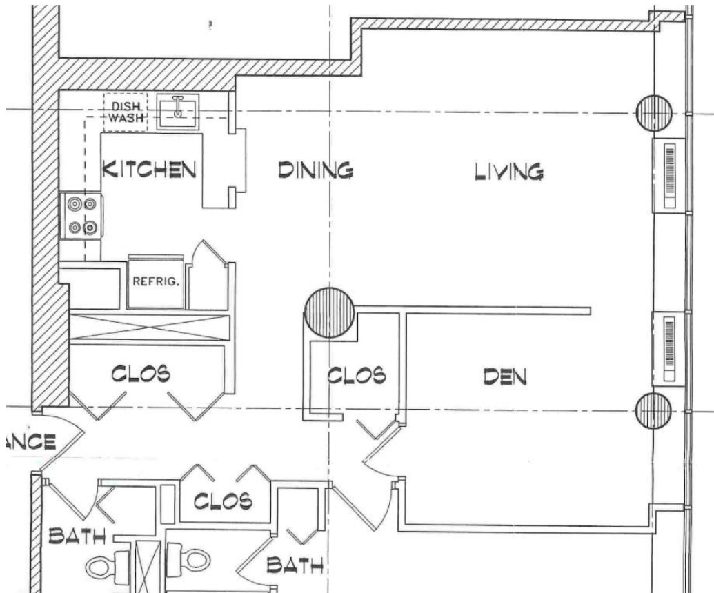
ORIGINAL FLOOR PLAN
